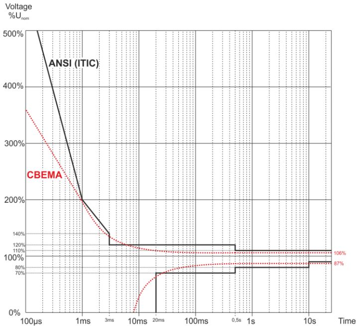
Fig. 21. Voltage tolerance curves ANSI (ITIC) and CBEMA.
