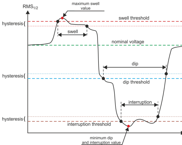
Fig. 19. Voltage swells, dips and interruptions.
