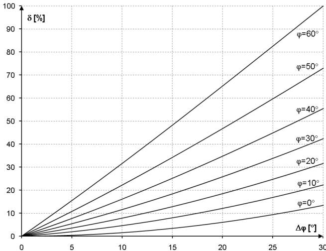
Fig. 24. Additional uncertainty from phase error depending on phase shift angle.
