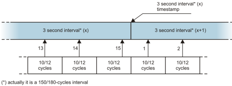
Fig. 23. Determining the averaging intervals shorter than 10 seconds (with the 3-second averaging).
