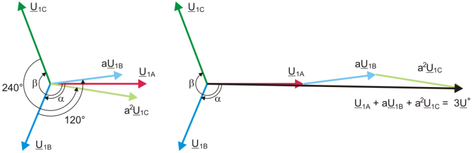
Fig. 18. Example of determination of positive sequence component.
