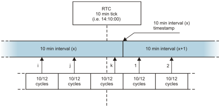
Fig. 22. Determining the averaging intervals equal to or longer than 10 seconds (with the 10-minute averaging).
