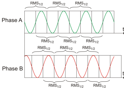
Fig. 20. Determination of the U_{rms(1/2)} value.
