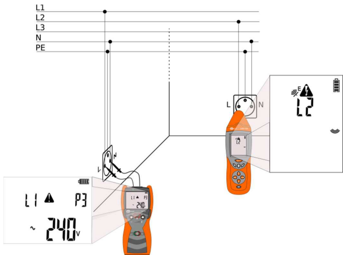
Fig. 31 Phase identification.
