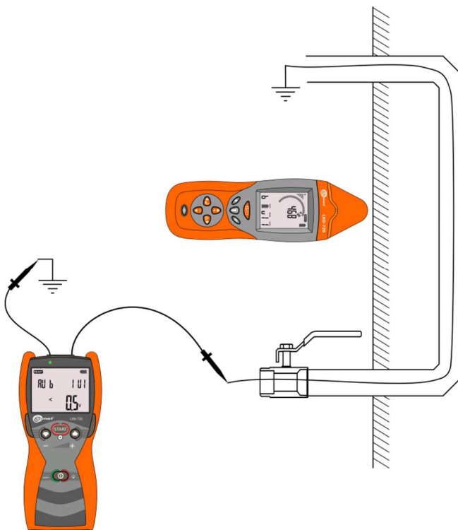
Fig. 30 Tracing electrically non-conductive hydraulic system.
