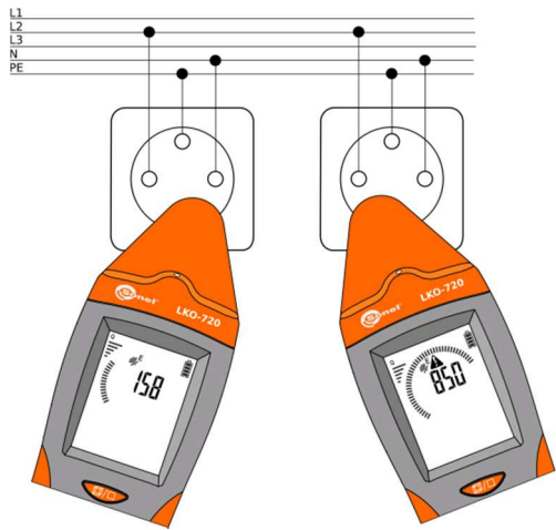
Fig. 32 Detecting electric field.
