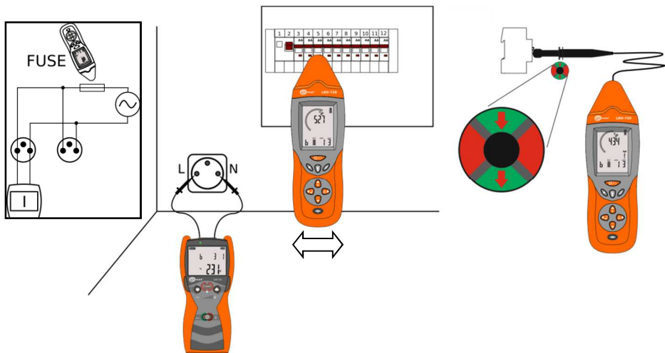
Fig. 27 Identifying safety devices in a switchboard.
