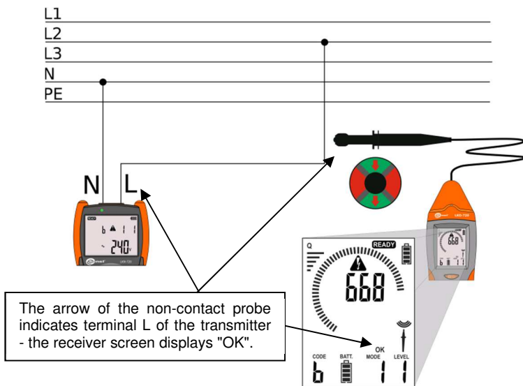
Fig. 41 Non-contact probe - the identification of the terminal L of the transmitter.
