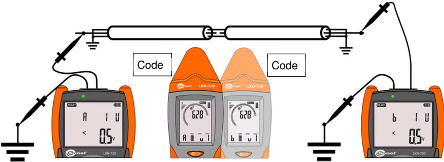
Fig. 33 Locating breaks – multi-transmitter mode.
