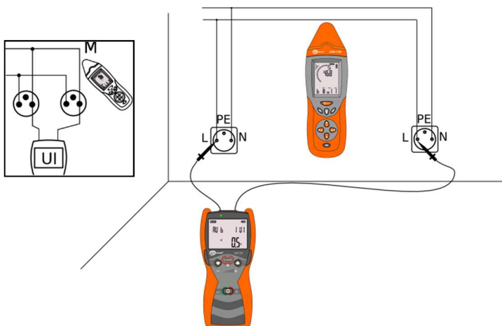
Fig. 24 Locating electrical system using a close loop.
