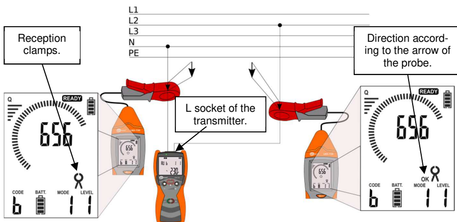
Fig. 37 Reception clamps – current forcing in detected circuit.
