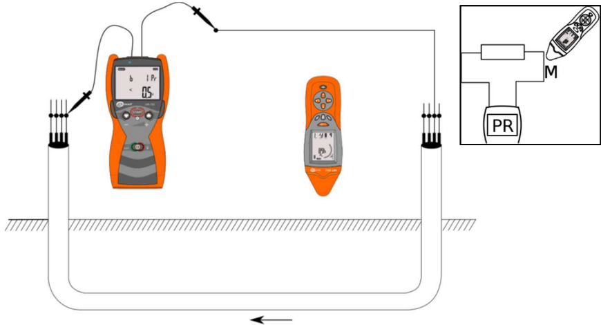
Fig. 29 Locating cables in Power mode using an external cable.
