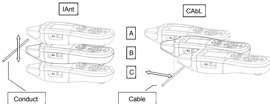
Fig. 19 Locating conductor/cable located in perpendicular to the symmetry axis of the receiver.
