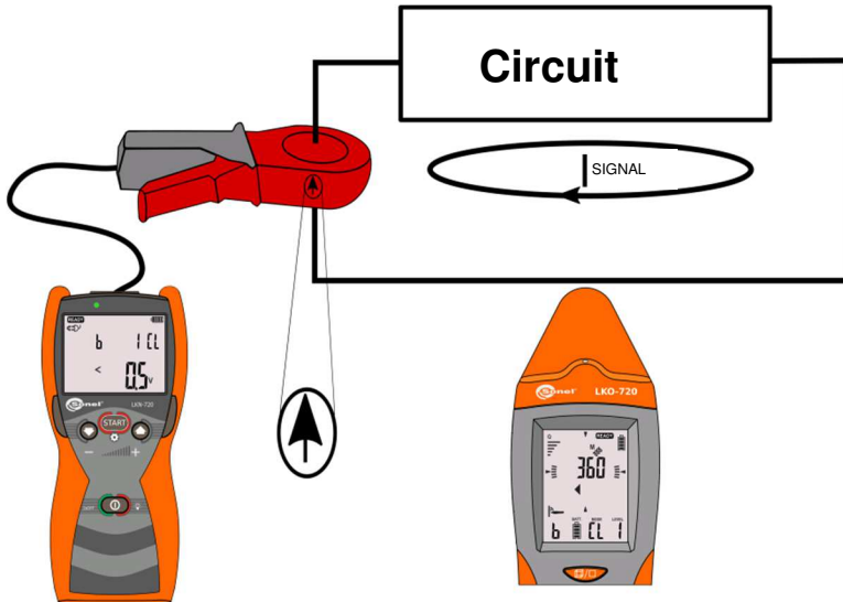
Fig. 36 Transmission clamps – current forcing in detected circuit.
