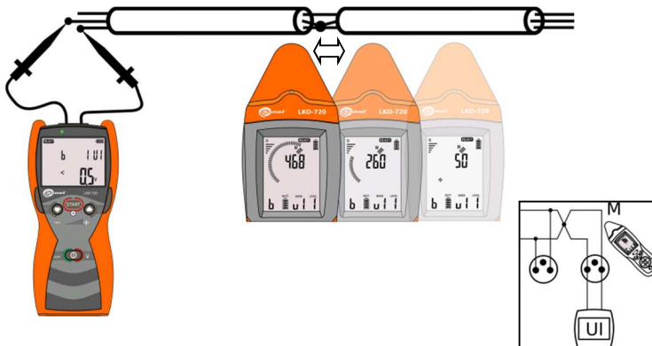
Fig. 26 Locating shorted cores in a conductor.
