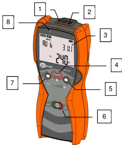
Fig. 1 Front panel.
