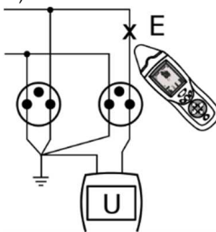
Fig. 8 Diagram of the voltage mode.
