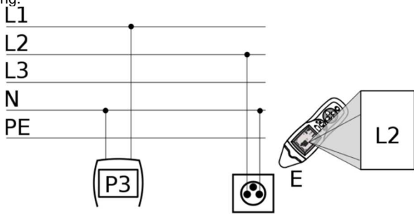
Fig. 10 Diagram of detecting P3 phase.
