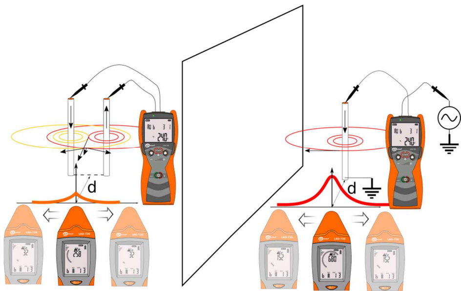
Fig. 18 Vectors of the magnetic field in two parallel conductors.
