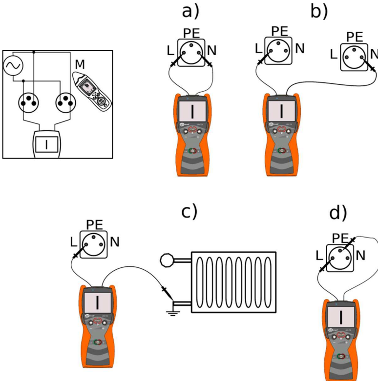
Fig. 17 Examples of connecting the transmitter to the electrical system.
