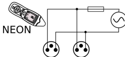
Fig. 14 Diagram of detecting 50Hz/60Hz electric field.
