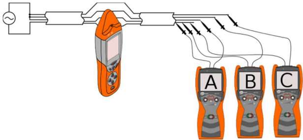
Fig. 34 Identifying cores in the cable – mode I.
