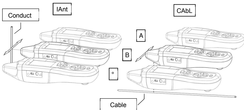
Fig. 20 Locating conductor/cable located in parallel to the symmetry axis of the receiver.
