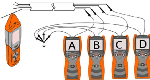
Fig. 35 Identifying cores in the cable – mode U.
