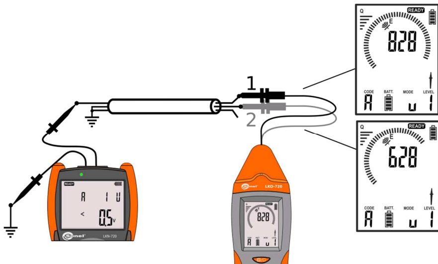
Fig. 38 Contact probe – identifying conductors.
