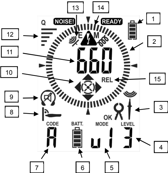
Fig. 4 Rreceiver - LCD display.
