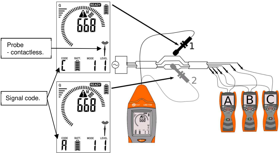
Fig. 40 Non-contact probe – identifying conductors during multi-transmitter operation.
