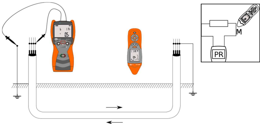
Fig. 28 Locating cables in power mode with shorted cores of the cable.
