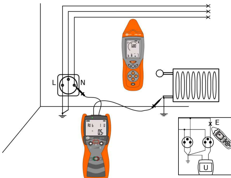
Fig. 23 Locating conductors disconnected from the network in the wall.
