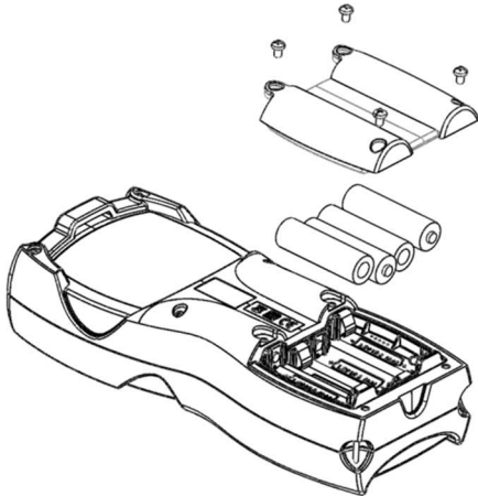
Fig. 16 Transmitter - battery replacement.
