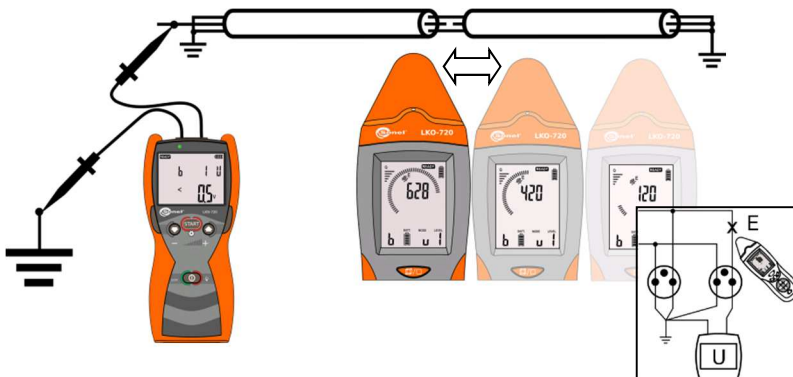
Fig. 25 Locating breaks.
